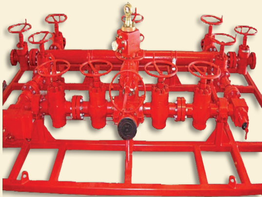
CHOKE & KILL MANIFOLD
